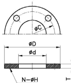
SEAT FLANGE
